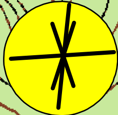
HQ Measured Bedrock Fracture Orientations
